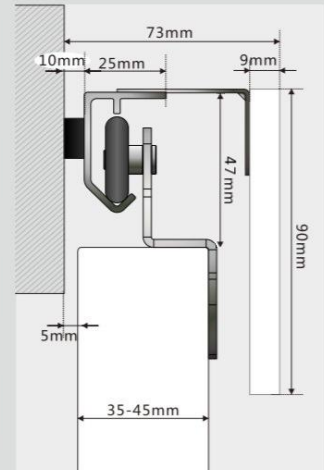
Hang Roller TY2.062.023.08
